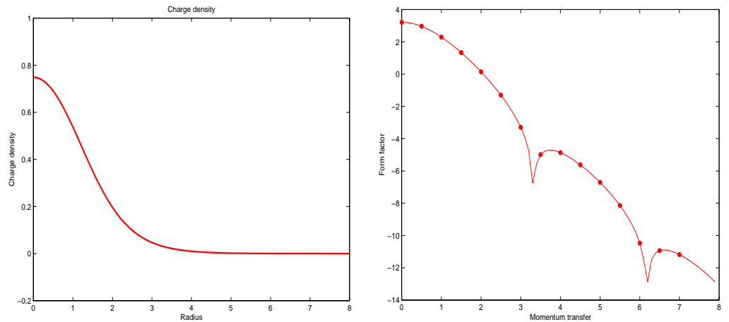
Fig. 6: Theoretical charge density \rho(r) , charge form factor \log |F(q)| and the data [stars] used for numerical experiments [right].
